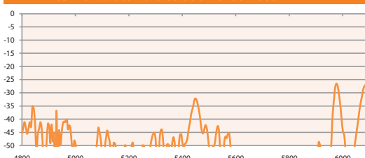
Antenna Port to Port Isolation 6100-4800 MHz
