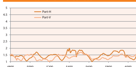
Antenna VSWR 6100-4800 MHz
