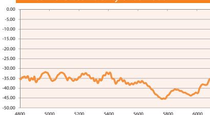
Antenna Cross Polarity 6100-4800 MHz
