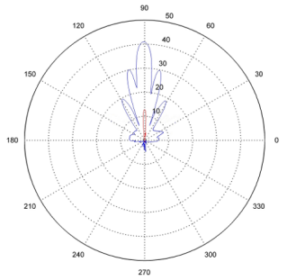
5.5 Ghz E-Plane and H of E-plane
