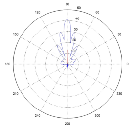
5.5 Ghz E-Plane and H of E-plane
