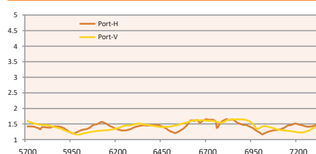
Antenna VSWR 5700-7200 MHz
