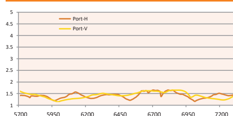
Antenna VSWR 5700-7200 MHz
