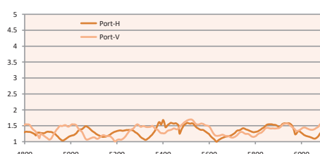
Antenna VSWR 4800-6100 MHz
